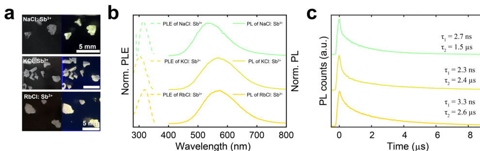
Fig. 2 (a) Optical images of \text{Sb}^{3+} -doped ACl ( A = \text{Na}, \text{K}, \text{and Rb} ) single crystals under ambient and UV light (254 nm). (b) Solid lines: PL emission spectra of \text{Sb}^{3+} -doped ACl ( A = \text{Na}, \text{K}, \text{and Rb} ). Dashed lines: PLE spectra of the same materials. (c) Time-resolved PL decay curves of \text{Sb}^{3+} -doped ACl ( A = \text{Na}, \text{K}, \text{and Rb} ) single crystals.
