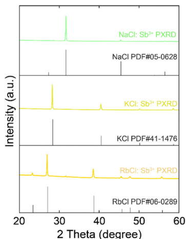
Fig. 1 PXRD pattern of \text{Sb}^{3+} -doped ACl ( A = \text{Na}, \text{K}, \text{and Rb} ) single crystals compared to standard XRD patterns PDF# 05-0628 of NaCl, PDF# 41-1476 of KCl, and PDF# 06-0289 of RbCl.
