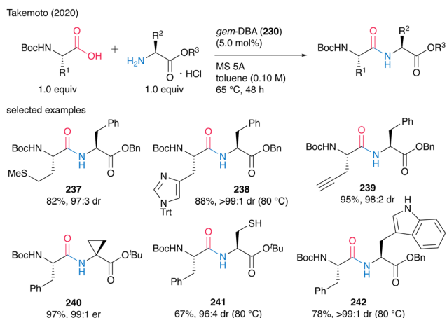
Scheme 51 gem -DBA-catalyzed dipeptide synthesis reported by Takemoto. 59
