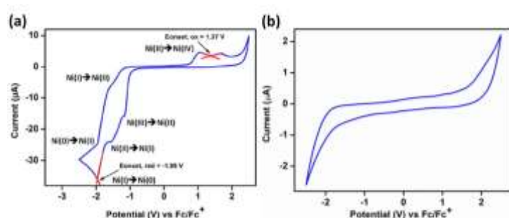
Fig. 14 CV of complex 62 in \text{CH}_2\text{Cl}_2 (a) and ligand 61 in THF (b), with 0.05 M t -butylammonium-hexafluorophosphate. All potentials were referenced to the \text{Fc/Fc}^+ couple. Scan rate = 50 \text{ mV s}^{-1} . Reproduced from Ref [35] Copyright © 2022, American Chemical Society.
