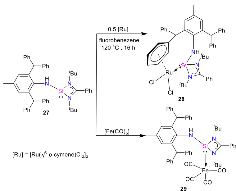
Scheme 9 Synthesis of 28 and 29 .
