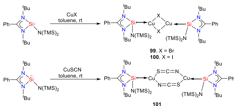
Scheme 38 Synthesis of Cu(I) complexes 99-101 .
