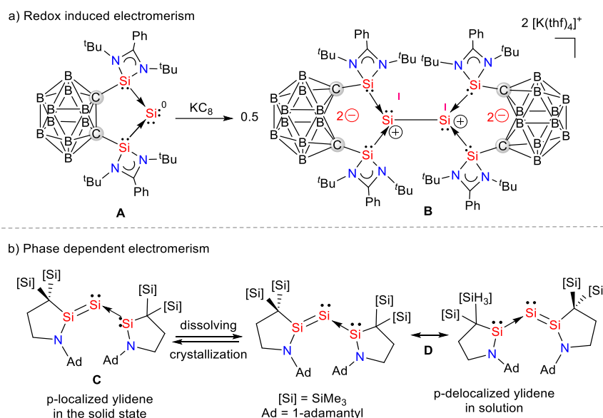
Scheme 35 Valence tautomerism in low-valent silicon chemistry.
