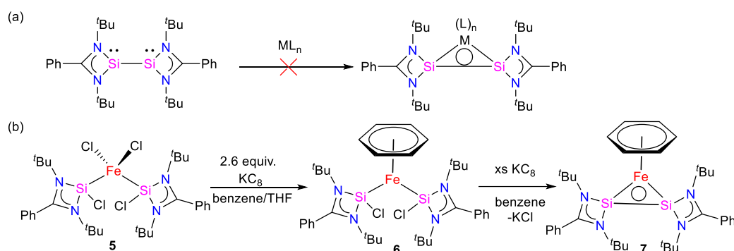
Scheme 2 (a) Non-reactivity of interconnected bis(silylene) for the formation of mononuclear metal adduct to Si–Si bond (b) Synthetic of complex 7.
