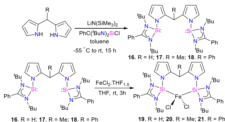
Scheme 6 Synthesis of 16–18 and iron chloride complexes 19–21 .
