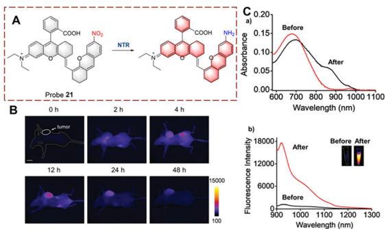
Fig. 22 (A) The structure and response mechanism of probe 21 . (B) Images of probe 21 in A549 tumour-bearing mice. (C) The absorbance spectra (a) and fluorescence spectra (b) of probe 21 before and after reduction (reprinted with permission from ref. 78 Copyright © 2021, Royal Society of Chemistry).
