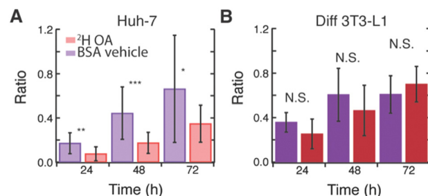
Fig. 4 Effect of OA feeding on rates of de novo lipid storage. Ratio of 13 C lipid to 12 C lipid in live (A) Huh-7 and (B) 3T3-L1 cells fed with both 2 H oleic acid and 13 C glucose (red) or BSA vehicle and 13 C glucose (purple) at 24, 48, and 72 h. N = 8–16 cells per time point * p -value < 0.05 ** p -value < 0.005 *** p -value < 0.0005 N.S. p -value > 0.05.
