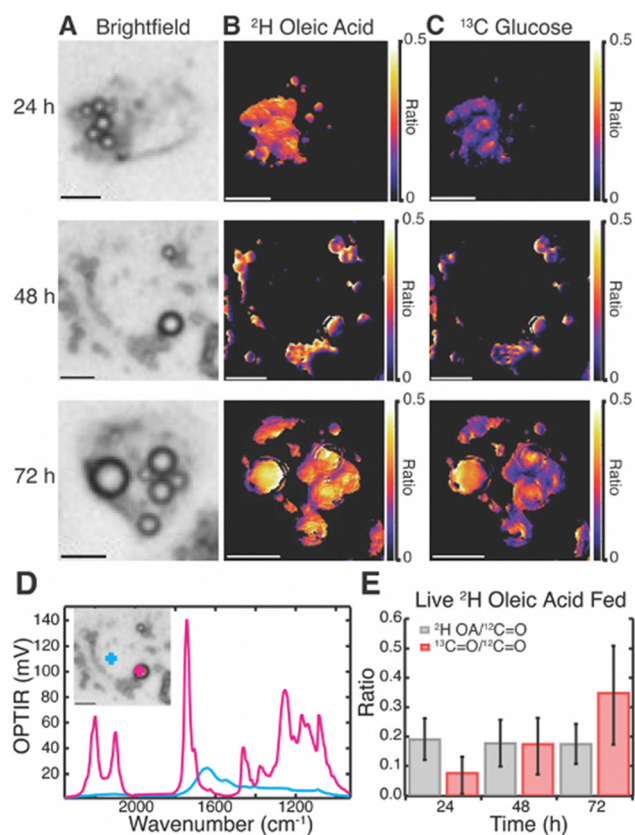
Fig. 3 Visualization of rates of glucose-derived de novo lipid storage in live Huh-7 cells fed with both 2 H OA (60 μM) and 13 C glucose (4.5 mg mL -1 ). (A) Brightfield images of live cells. (B) 2 H OA ratio images of 2 H lipid to the 12 C lipid band, after correction. (C) 13 C glucose ratio images of the 13 C lipid band to the 12 C lipid band, after correction. (D) Representative spectra of the live Huh-7 cell at the 48-hour time point both inside a LD (pink) and outside the droplet (blue). (E) Average ratios of 2 H lipid band (grey) and 13 C lipid band (red) to 12 C lipid band across many cells (N = 14). Scale bars are 10 μm.
