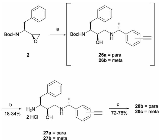
Scheme 6 Synthesis of probes 20b and 20c . Reagents and conditions: (a) Amines 25a/25b , \text{Et}_3\text{N} , MeOH, 65^\circ\text{C} , o/n; (b) HCl 4 M in dioxane, DCM, r.t., o/n; (c) 4-benzoylbenzoic acid 21 , HATU, 4-ethylmorpholine, DMSO, r.t., o/n.
