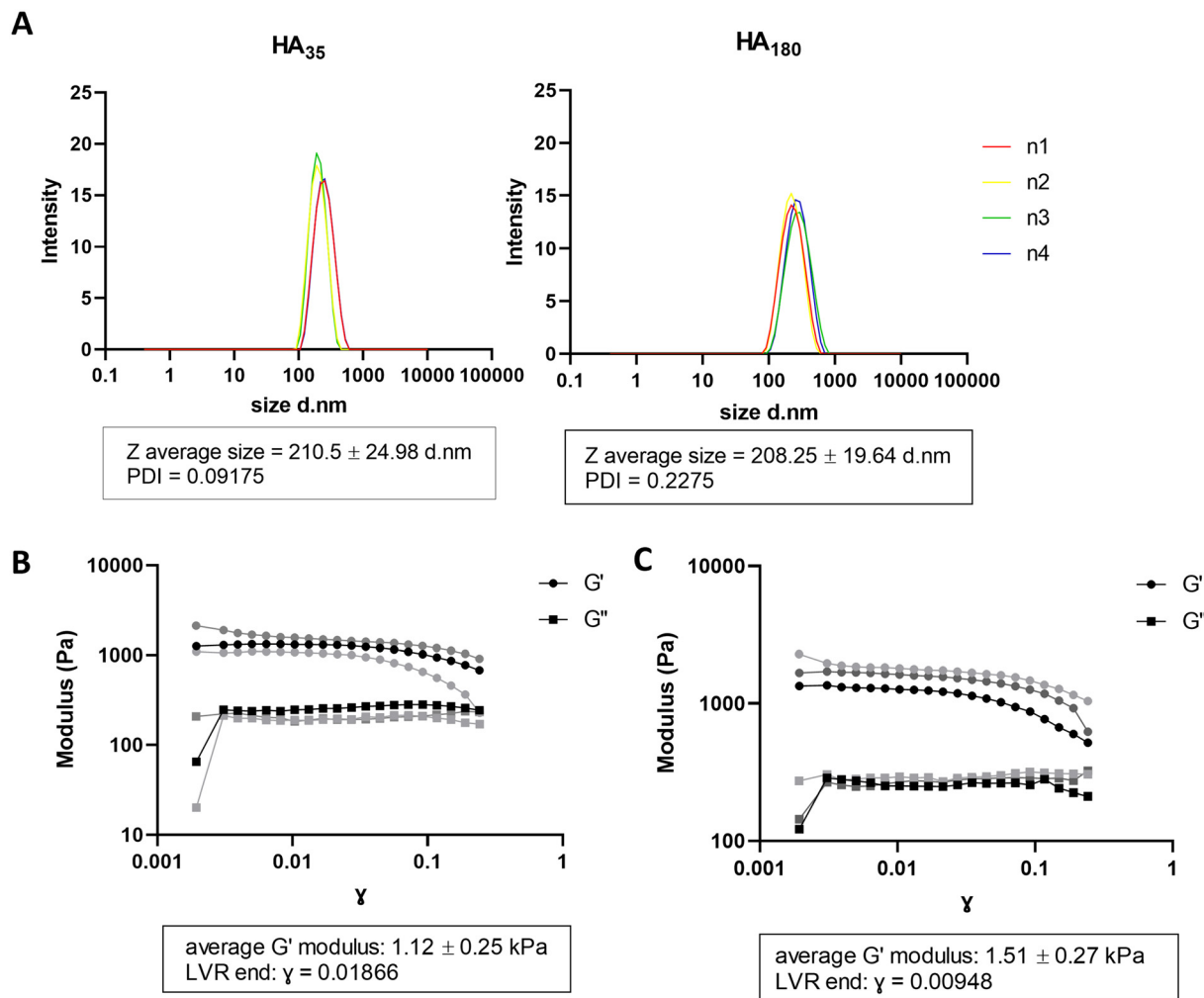
Fig. 2 Hyaluronic acid/chitosan nanoparticles incorporated into alginate cell forms a layer with a similar stiffness to brain tissue. (A) Dynamic light scattering measurements of HA 35 /CS and H 180 /CS nanoparticles, n = 4 independent repeats. (B) Shear moduli for A4 HA 35 /CS hydrogel crosslinked using 75 mM CaCl 2 solution (aq.) ( n = 3 independent repeats) (C) Shear moduli of A4 HA 180 /CS hydrogel crosslinked using 75 mM CaCl 2 ( n = 3 independent repeats). PDI: polydispersity index, LVR: linear viscoelastic region, G': elastic modulus, G'': viscosity modulus.
