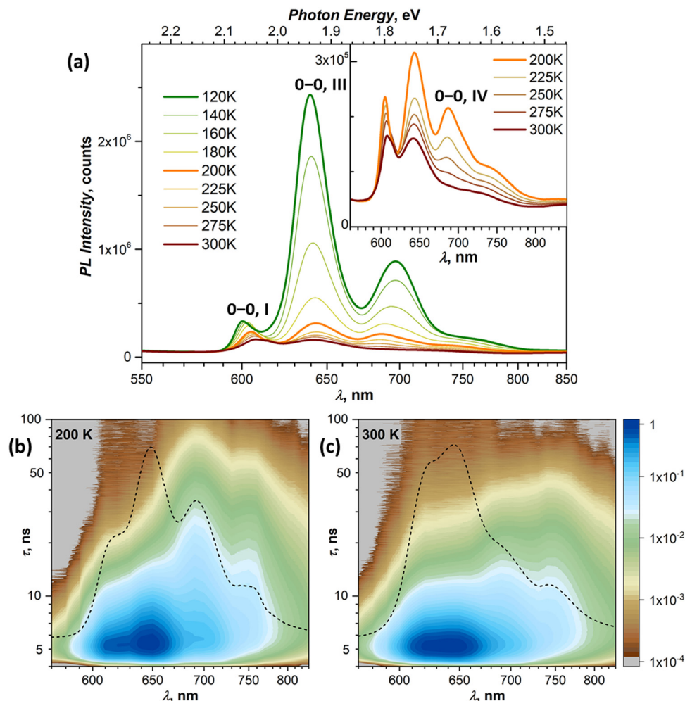
Fig. 4 (a) VT-PL spectra of DBP in the temperature range of 120–300 K; (b) and (c) ( \lambda , \tau ) maps of the PL decay at 200 K (b) and 300 K (c); note that the laser pulse occurs at \tau = 4 ns and the time after pulse and PL intensity are given in log scale; each map is overlaid by a quasi-CW TR spectrum (dashed curve), obtained by integration of PL decay over 100 ns after the pulse. Note that some of the features observed in the CW spectra are smeared in the TR spectra because of the lower resolution.
