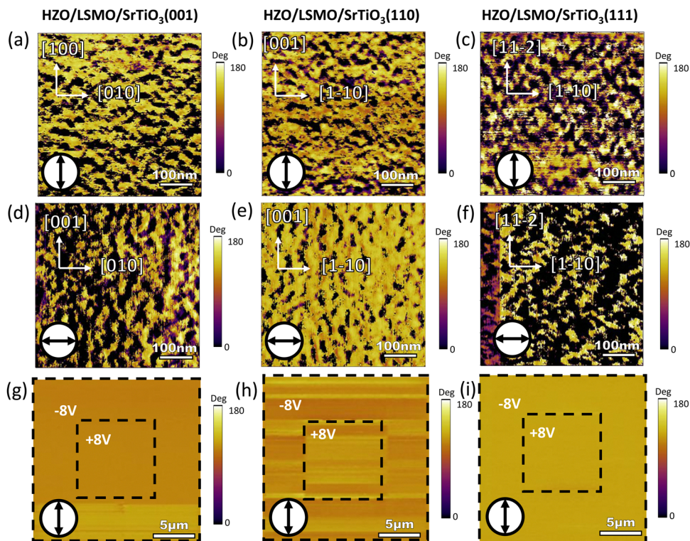
Fig. 4 (a–c) PFM in-plane phase images for the three HZO films grown on LSMO/SrTiO 3 (001), LSMO/SrTiO 3 (110) and LSMO/SrTiO 3 (111), respectively. Response is probed along the vertical in-plane direction as indicated in the inset. (d–f) Idem, while probing along the horizontal in-plane direction. (g–i) PFM in-plane phase images for the three HZO films after applying + and –8 V in the inner and outer regions as indicated. The in-plane substrate orientation in (g–i) is the same as in (a–c).
