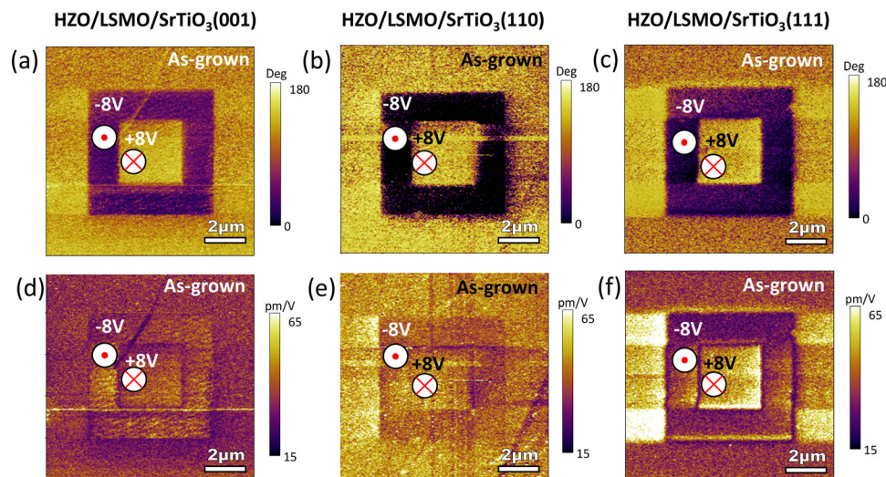
Fig. 3 (a–c) PFM out-of-plane phase images for the three HZO films grown on LSMO/SrTiO 3 (001), LSMO/SrTiO 3 (110), and LSMO/SrTiO 3 (111), respectively, after applying +/–8 V in the bright (dark) regions. The outer region corresponds to the as-grown state and no voltage has been applied. (d–f) PFM out-of-plane amplitude images corresponding to the (a–c) phase image regions.
