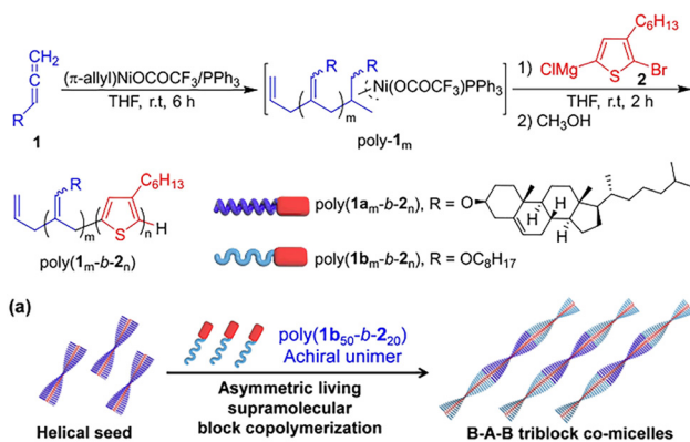
Fig. 13 Synthesis of P3HT block copolymers (top). Schematic illustration of asymmetric living supramolecular block copolymerization of achiral poly(1b 50 - b -2 20 ) unimer initiated by right-handed helical seed micelle of poly(1a 80 - b -2 20 ) (down). Copyright 2022, WILEY-VCH.
