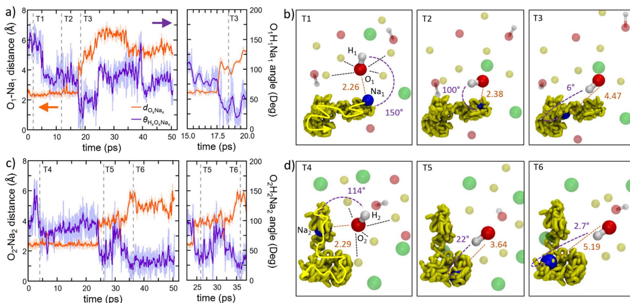
Fig. 9 (Color online) Proposed paddlewheel dynamics monitored in amorphous Na 2.5 OH 0.5 Cl at 300 K. We show the temporal evolutions of two distinct scenarios involving different atoms. (a and c) The interatomic distance between an O atom (O 1 and O 2 ) of one hydroxyl group and a coordinated Na atom (Na 1 and Na 2 ) and the HONa angles (H 1 O 1 Na 1 and H 2 O 2 Na 2 ) along the ~50 ps trajectory. Light orange and purple lines correspond to the instantaneous interatomic distance d_{O_xNa_x} and \theta_{H_xO_xNa_x} angle, whereas the strong lines correspond to the sliding average with a window of 0.1 ps. (b and d) Atomistic views of the temporal frames T y ( y = 1-6 ) indicated in (a) and (b). In (b), between 0 and 5 ps, a sixfold coordinated O 1 atom of one hydroxyl group shows a bonding distance of 2.26 Å with the Na atom labelled Na 1 and an HONa angle of ~150° (T 1 ). At 5 ps, the hydroxyl OH bond is rotating with respect to Na 1 (from ~150° to ~100°) while maintaining a distance O 1 -Na 1 equal to 2.38 Å. This scenario lasts up to 17 ps (T 2 ). After 17.5 ps and up to 25 ps a further rotation of the OH group bringing the corresponding angle from ~100° to ≤50° (~6° at T 3 ) induces the displacement of the Na 1 atom to a larger distance (>4.5 Å) escaping the first coordination shell of the O 1 atom. In (d) between 4 and 23 ps, a sixfold coordinated O 2 atom of one hydroxyl group shows a bonding distance of 2.29 Å with the Na atom labelled Na 2 and an HONa angle of 90°–120° (T 4 ). At 26 ps, the hydroxyl OH bond is rotating with respect to Na 2 (to ≤50°) inducing the displacement of the Na 2 atom to a larger distance (>3.6 Å) escaping the first coordination shell of the O 2 atom (T 5 ). A further rotation to 3° is accompanied by a displacement of the Na 2 atom to a larger distance (>5 Å, T 6 ). The surrounding atoms of O 1 and O 2 at a distance lower than >5 Å are shown in transparent color. Dashed lines indicate the atoms coordinated within the first coordination shell of O 1 and O 2 (<3.3 Å). The concerted migration pathways of Na 1 and Na 2 atoms along the ~50 ps trajectory are shown in transparent dark yellow. As a guide, an arrow is added to indicate the direction of the pathway. Color legend: Na atoms, yellow; O atoms, red; Cl atoms, green; H atoms, white; Na 1 and Na 2 atoms at T y points are shown in blue.
