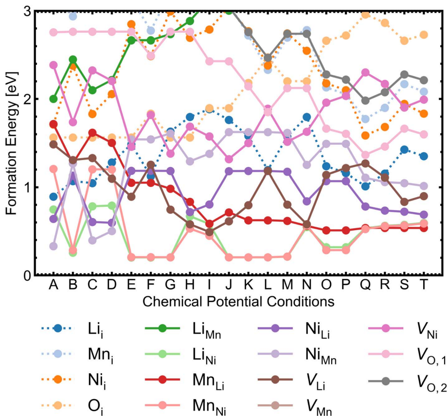
Fig. 4 Formation energies for each intrinsic point defect in the lowest energy charge state at the self-consistent Fermi levels over 20 chemical potential conditions for P_{4/3}3/2 \text{LiMn}_{1.5}\text{Ni}_{0.5}\text{O}_4 . The chemical potential conditions (A \rightarrow T) are arranged in order of increasing self-consistent Fermi level determined from all intrinsic point defects. Interstitial defects are represented by dotted lines; antisite and vacancy defects are shown by solid lines.
