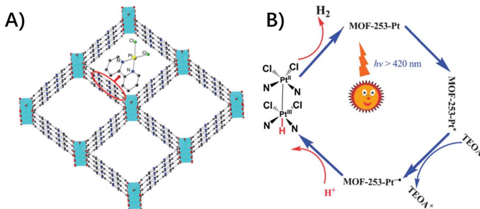
Fig. 10 (A) A model structure of MOF-253-Pt through the post-synthetic modification of MOF-253 with \text{PtCl}_2 . (B) A proposed reaction mechanism via pairs of dichloro-platinum(II) complexes for the photocatalytic \text{H}_2 evolution. Reproduced from ref. 42 with permission from the Royal Society of Chemistry.
