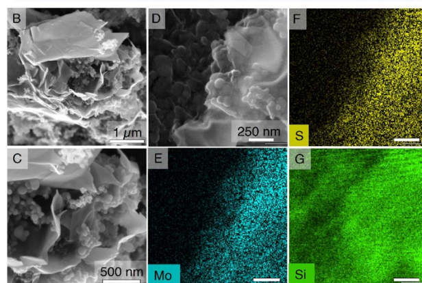
Fig. 3 Preparation and analysis of the MoS 2 @Si heterostructure composite. (A) The schematic illustrates the preparation method of the heterostructure through layer-by-layer addition of MoS 2 and Si via vacuum filtration. (B–D) The SEM and (E–G) EDS images of the MoS 2 @Si heterostructure depict various elements in the composite structure.
