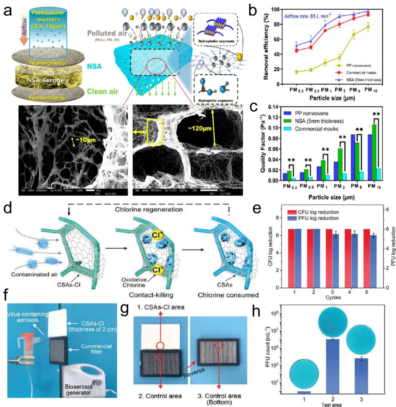
Fig. 13 3D fibrous aerogels used in air filtration. (a) Illustration of the contaminants captured by SNF aerogels. (b) Removal efficiency at 85 L \text{min}^{-1} for differently sized particles. (c) Quality factor of the three kinds of materials at 85 L \text{min}^{-1} for differently sized particles. Reproduced with permission. 88 Copyright 2021, American Chemical Society. (d) Illustration showing the air filtration procedure of the aerogels. (e) Renewable antibacterial and antiviral properties of CSAs-Cl. (f) Virus-containing aerosol generator and the antiviral test using an aerogel and 3 M filter. (g and h) The antiviral properties of the selected three areas of the filters. Reproduced with permission. 92 Copyright 2021, Wiley-VCH.
