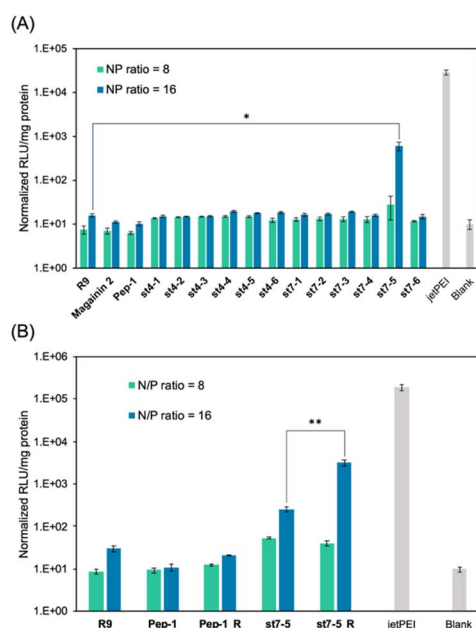
Fig. 2 Transfection efficiency of stapled peptides and R9/pDNA complexes after a 24 h incubation in HeLa cells. The relative light unit (RLU) of (A) stapled peptides/pDNA complexes and (B) these derivatives with Lys substituted Arg, the transfected rLuc pDNA was normalized by the blank. N/P ratio = 8 (green) and 16 (blue), n = 3 , mean \pm standard deviation. Symbols (*) indicate statistical significance (* p < 0.05 and ** p < 0.02 ).
