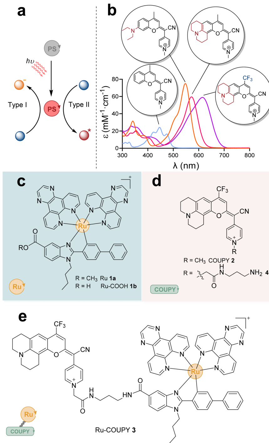
Fig. 1 Rational design of Ru-COUPY conjugate for anticancer PDT. (a) Electron- (Type I) and energy-transfer (Type II) mechanisms of PDT. (b) Tunability of the coumarin scaffold and UV-vis absorption spectra of some COUPY fluorophores. (c–e) Structures of the investigated compounds: Ru(II) complexes ( 1a and 1b ), COUPY coumarins ( 2 and 4 ) and Ru-COUPY conjugate ( 3 ).
