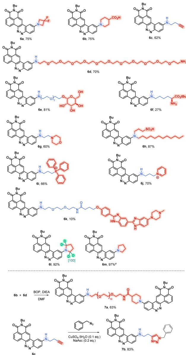
Fig. 4 Examples of accessible original CinNaphhts using S_NAr late-stage functionalization with isolated yields. a Compound described previously 5 and accessible thanks to the S_NAr late-stage functionalization.
