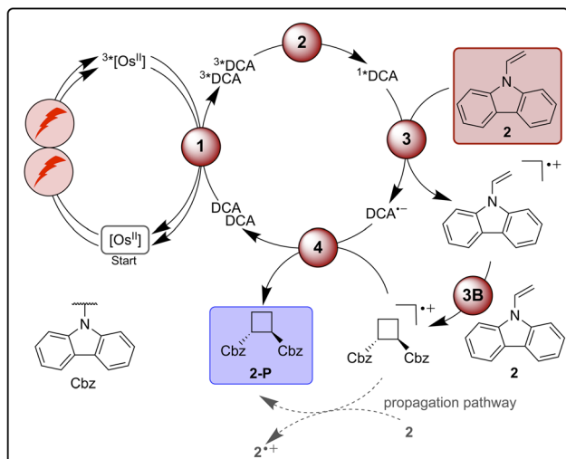
Fig. 4 [2 + 2] Cycloaddition of vinylcarbazole ( 2 ) under red-light irradiation and a plausible mechanism involving triplet-triplet energy transfer (1), triplet-triplet annihilation upconversion (2), substrate activation (3), cycloaddition (3B), and catalyst recovery (4). Main steps of substrate activation adapted from a previously reported monophotonic mechanism. 106,115,116 A radical chain propagation pathway is likely for this reaction (details in text and ESI Section 4.8.3†). 106 The yield (conversion in parenthesis) was determined by 1 H-NMR spectroscopy using 1,4-dioxane as internal standard. Further information is in Section 4.5 of the ESI.† a Product isolation was performed on a 400 \mu\text{mol} scale of 2 under 623 nm LED irradiation.
