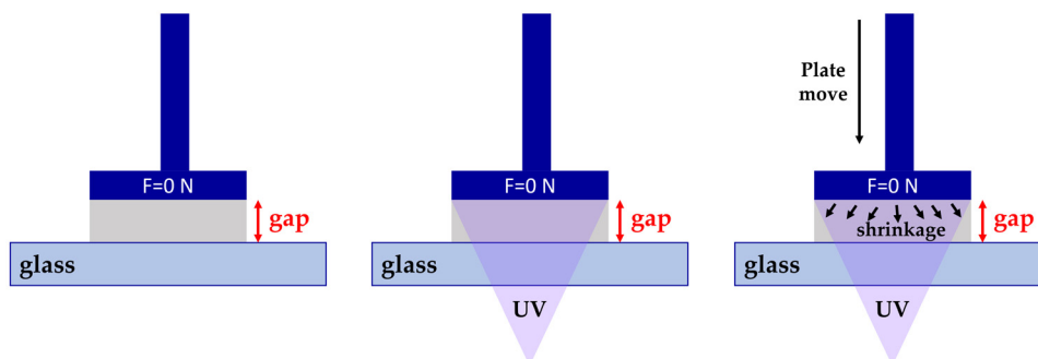
Fig. 15 Schematic representation of the shrinkage measurement apparatus.
