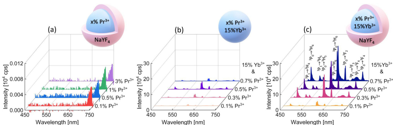
Fig. 2 Anti-Stokes emission spectra of \beta -NaYF 4 nanocrystals: (a) core–shells singly doped with Pr 3+ ions; (b) cores co-doped with x\%Pr^{3+} , 15%Yb 3+ ; (c) x\%Pr^{3+} , 15%Yb 3+ co-doped cores with a passive shell with assigned transitions. The presented emission spectra were recorded under 852 nm excitation (1.5 MW cm -2 ) at room temperature.
