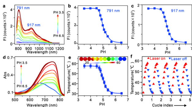
Fig. 1 Photophysical and photothermal properties of IR-PE. (a) Emission spectra of 5 \mu g mL^{-1} IR-PE at various pH values upon excitation at 750 nm. (b) Fluorescence intensity of IR-PE at 791 nm and (c) 917 nm in PBS with different pH values. (d) UV-Vis spectra of 5 \mu g mL^{-1} IR-PE at various pH values in PBS buffer. (e) Temperature curves of 10 \mu g mL^{-1} IR-PE in PBS with different pH values after continuous laser irradiation for 10 minutes. Inset: photothermal images of IR-PE in PBS with different pH values after continuous laser irradiation for 10 minutes (pH values in b–e: 3.5, 4, 4.5, 4.7, 4.8, 4.9, 5, 5.1, 5.2, 5.4, 5.7, and 6.5). (f) The photothermal stability study of 10 \mu g mL^{-1} IR-PE in PBS (pH 3.5) by repeated 808 laser irradiation for 5 cycles (10 min of laser on and then naturally cooled to room temperature in each cycle).
