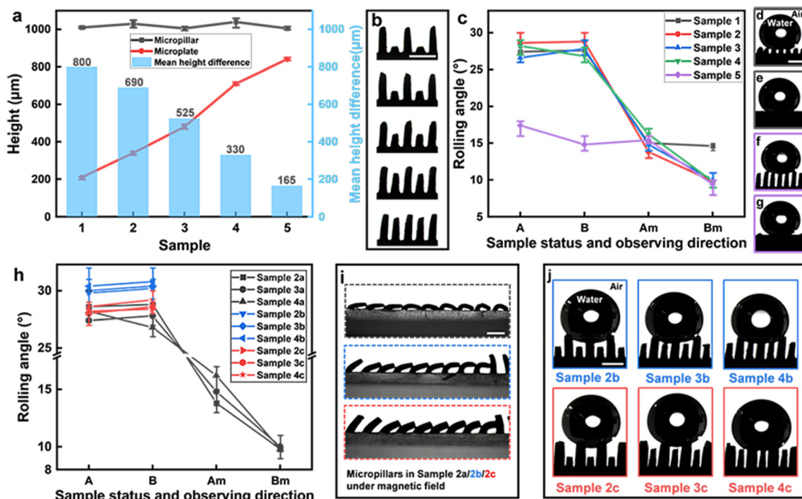
Fig. 4 (a) Height and height difference of the micropillars and microplates on samples 1–5. (b) Photographs of samples 1–5 observed along the direction A. (c) Rolling angles of water droplets on samples 1–5 without/with a magnetic field along directions A and B. Static contact situations of water droplets on sample 1 along directions A and B: (d) and (e) with a magnetic field, (f) and (g) without a magnetic field. (h) Rolling angles on samples 2a–4c along directions A and B without/with a magnetic field. (i) Micro-pillar bending behaviors of samples 2a, 2b, and 2c under a magnetic field. (j) Contact situations on samples 2b–4c along direction A without a magnetic field. Droplet volume = 10 \mu\text{L} , scale bar = 1 mm.
