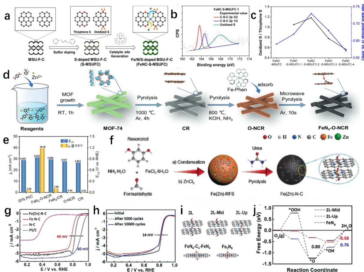
Fig. 9 (a and b) Schematic representation of the synthesis and S 2p XPS spectra of FeNC–S–MSUFC. (c) Relationship between the ratio of oxidized S and thiophene-like S and ORR activity. Reproduced with permission ref. 133. Copyright 2019, American Chemical Society. (d and e) Scheme of the synthesis, E 1/2 and j k of the FeN 4 –O–NCR. Reproduced with permission ref. 77. Copyright 2022, Wiley-VCH. (f–i) Synthesis, LSV curves, the durability tests, and illustration of proposed various structures of Fe(Zn)–N–C. (j) Gibbs free energy diagrams at 1.23 V on FeN 4 , 2L–Mid, and 2L–Up sites. Reproduced with permission ref. 134. Copyright 2020, Wiley-VCH.
