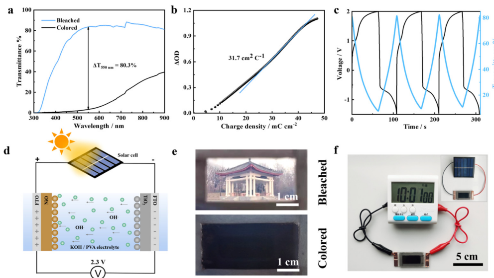
Fig. 5 Electrochromic performances of a self-powered smart window: (a) optical transmittance spectra in the colored and bleached states; (b) the changes of optical density with charge density at 550 nm; (c) GCD curve and the in situ transmission spectrum of the smart window at 0.65 \text{ mA cm}^{-2} ; (d) schematic diagram of the working principle of the photovoltaic electrochromic device; (e) digital photographs of the device ( 2.5 \times 5 \text{ cm}^2 ) in the colored and bleached states, respectively; and (f) a digital watch driven by the smart window (inset: the colored smart window driven by a solar panel).
