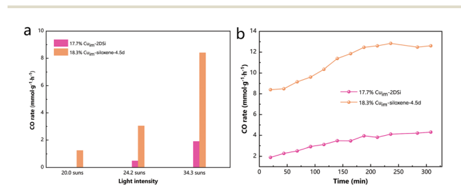
Fig. 3 CO rates of different samples in photothermal catalytic reactions (testing conditions: 15 mg of the catalyst, CO 2 /H 2 /N 2 = ~2.5/10/2.5, and ambient pressure).
