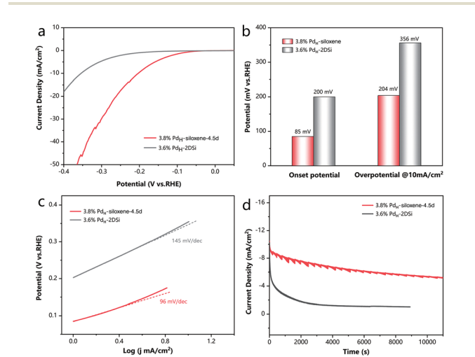
Fig. 4 (a) Polarization curves of the 3.6% Pd H -2DSi and 3.8% Pd H -siloxene-4.5d catalysts. (b) Comparison of the overpotential at 10 mA cm -2 and the onset potential of the catalysts. (c) Tafel plots of the catalysts. (d) Chronoamperometry tests of the catalysts.
