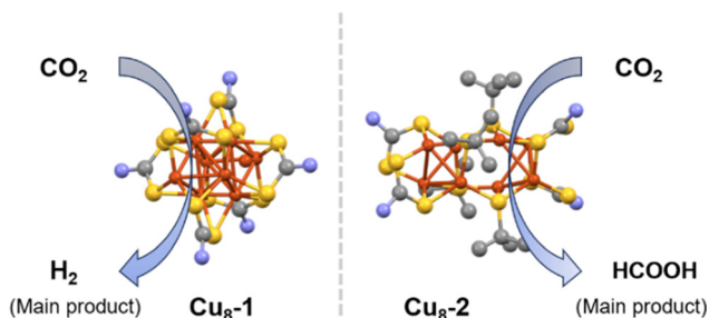
Fig. 9 Effect of the structural architecture of \text{Cu}_8 NC in selectivity of \text{CO}_2\text{RR} product formation. Cu displayed in brown color; S displayed in yellow color; N displayed in blue color and C displayed in light dark color. Other ligands were removed for clarity. Figure created based on the cif file deposition of ref. 81.
