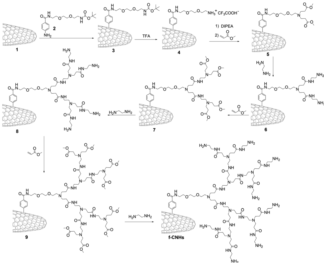
Scheme 1 Illustrative preparation of f-CNHS.
