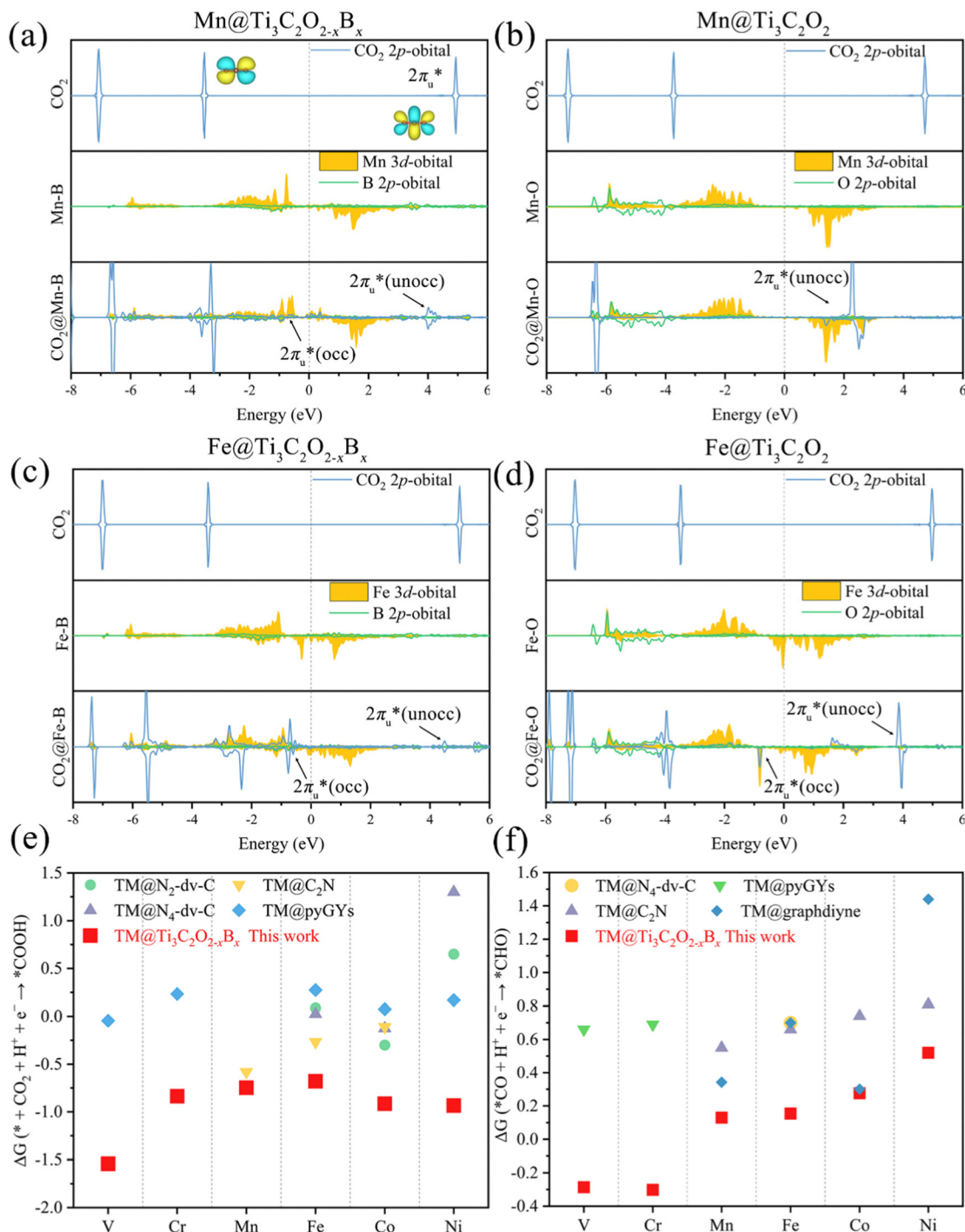
Fig. 3 The PDOS of CO 2 2p, TM 3d, and coordination atoms (the O atom in TM@Ti 3 C 2 O 2-x B x and the B atom in TM@Ti 3 C 2 O 2-x B x ) of the 2p orbital before and after CO 2 adsorption on (a) Mn@Ti 3 C 2 O 2-x B x , (b) Mn@Ti 3 C 2 O 2 , (c) Fe@Ti 3 C 2 O 2-x B x and (d) Fe@Ti 3 C 2 O 2 . A comparison of the Gibbs free energy changes of (e) the 1st (CO 2 + H + + e - → *COOH) and (f) the 3rd (CO + H + + e - → *CHO) hydrogenation reactions for TM@Ti 3 C 2 O 2-x B x and other SACs (TM@N 2 -dv-C, 74 TM@N 4 -dv-C, 74 TM@C 2 N, 75 TM@pyGYs, 76 and TM@graphdiyne 77 ) for the CO 2 reduction.
