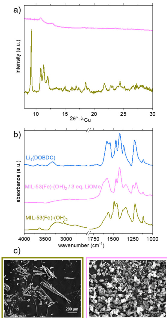
Fig. 5 Characterisation of \text{MIL-53}(\text{Fe})-(\text{OH})_2 and its lithiated product from LiOMe in MeOH/THF. a) PXRD patterns ( \lambda = 1.5406\text{ \AA} ); b) IR spectra; c) SEM pictures. Data related to dry \text{MIL-53}(\text{Fe})-(\text{OH})_2 , \text{Li}_4(\text{DOBDC}) and the lithiation product are shown in khaki, blue and pink, respectively.
