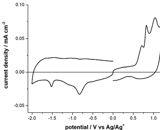
Fig. 2 Cyclic Voltammograms of DTDPAB molecule, in acetonitrile + 0.1 M Bu_4NClO_4 . Scan rate: 0.1 \text{ V s}^{-1} .
