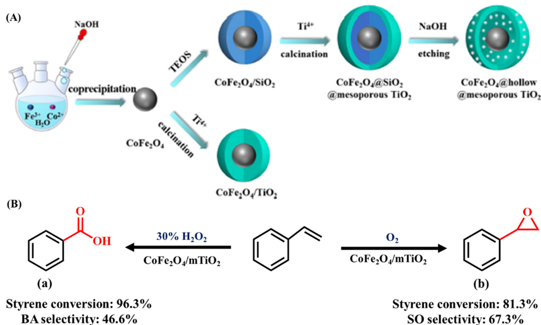
Scheme 19 (A) Procedure for the synthesis of \text{CoFe}_2\text{O}_4@hollow@mesoporous TiO_2 yolk-shell structure and \text{CoFe}_2\text{O}_4/\text{TiO}_2 core-shell structure and (B) application in styrene conversion. Reproduced with permission from ref. 138. Copyright 2020, the American Chemical Society.
