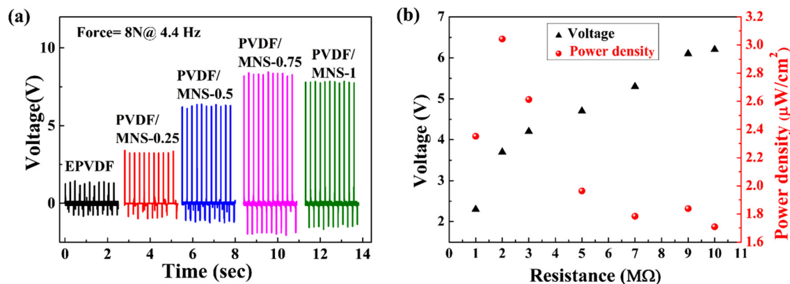
Fig. 11 (a) Piezoelectric response of EPVDF and PVDF/MNS composite nanofabrics-based PNG with varying loading of MNS, (b) piezoelectric voltage generated, and power density of PVDF/MNS-0.75 based PNG across the different resistances (applied force of 8 N).
