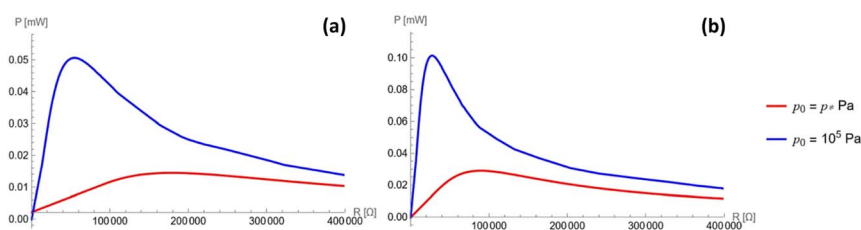
Fig. 5 Average power profile against the electric load for a flat electrode design. Curves are plotted for 2 stroke frequencies and gauge pressures for the flat electrode case, (a) \omega = 2\pi \text{ s}^{-1} and (b) \omega = 4\pi \text{ s}^{-1} each at gauge pressures p_0 = p^* and p_0 = 10^5 \text{ Pa} . Parameters: V_{\text{ref}} = 1 \text{ V} , \tilde{\gamma} = 3.44 \times 10^{-2} \text{ N m}^{-2} , \gamma_1 - \gamma_2 = 2.27 \times 10^{-2} \text{ N m}^{-2} , C_s = 0.1 \text{ F m}^{-2} , Q = 10^{-9} \text{ m}^3 , L = 0.1 \text{ m} , and H = 10^{-3} \text{ m} .
