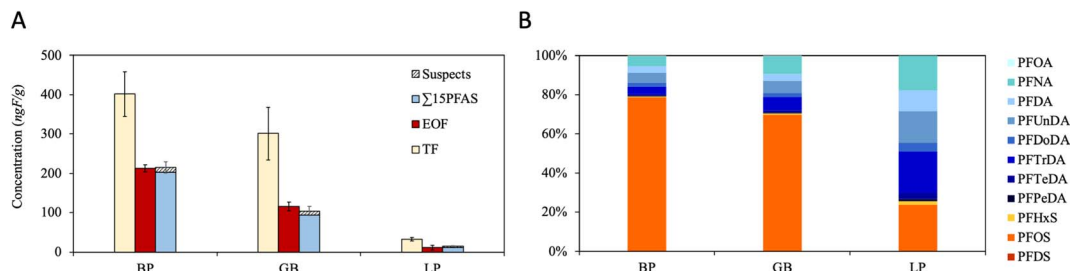
Fig. 4 (A) FMB detailing total fluorine (TF), extractable organofluorine (EOF), targeted PFAS ( \Sigma_{15} PFAS) and suspect concentrations ( \text{ng F g}^{-1} ) in pooled samples. PFHxA, PFHpA, and FOSA were not detected across all three regions and are therefore not shown. Error bars represent standard deviation of replicate analysis ( n = 3 ). (B) Normalised PFAS profiles of pooled samples. BP = Baltic Proper; GB = Gulf of Bothnia; LP = Northern Inland.
