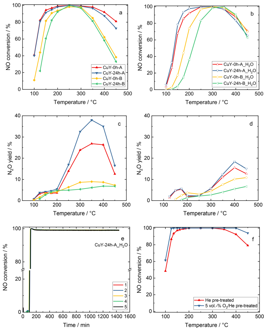
Fig. 10 a and b) NO conversion and c and d) N 2 O yield during NH 3 -SCR-DeNO x over copper-containing zeolite Y samples. Reaction conditions: m_K = 0.2 g; GHSV = 30 000 h -1 , c(\text{NO}) = 500 ppm, c(\text{NH}_3) = 575 ppm, c(\text{O}_2) = 4 vol%, ( c(\text{H}_2\text{O}) = 5 vol% when used), He balance, F_{\text{TOT}} = 120 ml min -1 , e) NO conversion over CuY-24h-A for five consecutive runs during the time-on-stream stability tests in the presence of water vapor at 200 °C, and f) NO conversion over CuY-24h-A after pre-treatment in He or 5 vol% O 2 /He.
