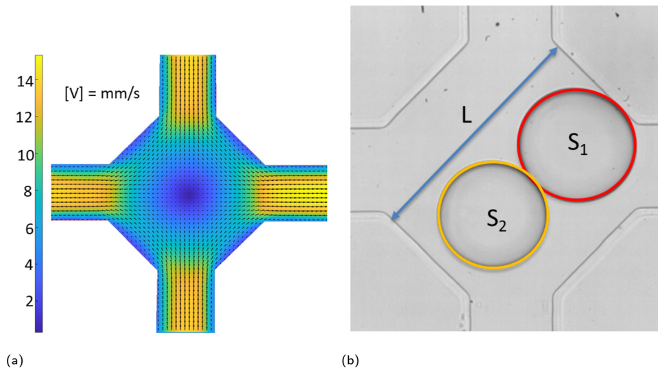
Fig. 1 Drop coalescence experiments in a microfluidic device.
