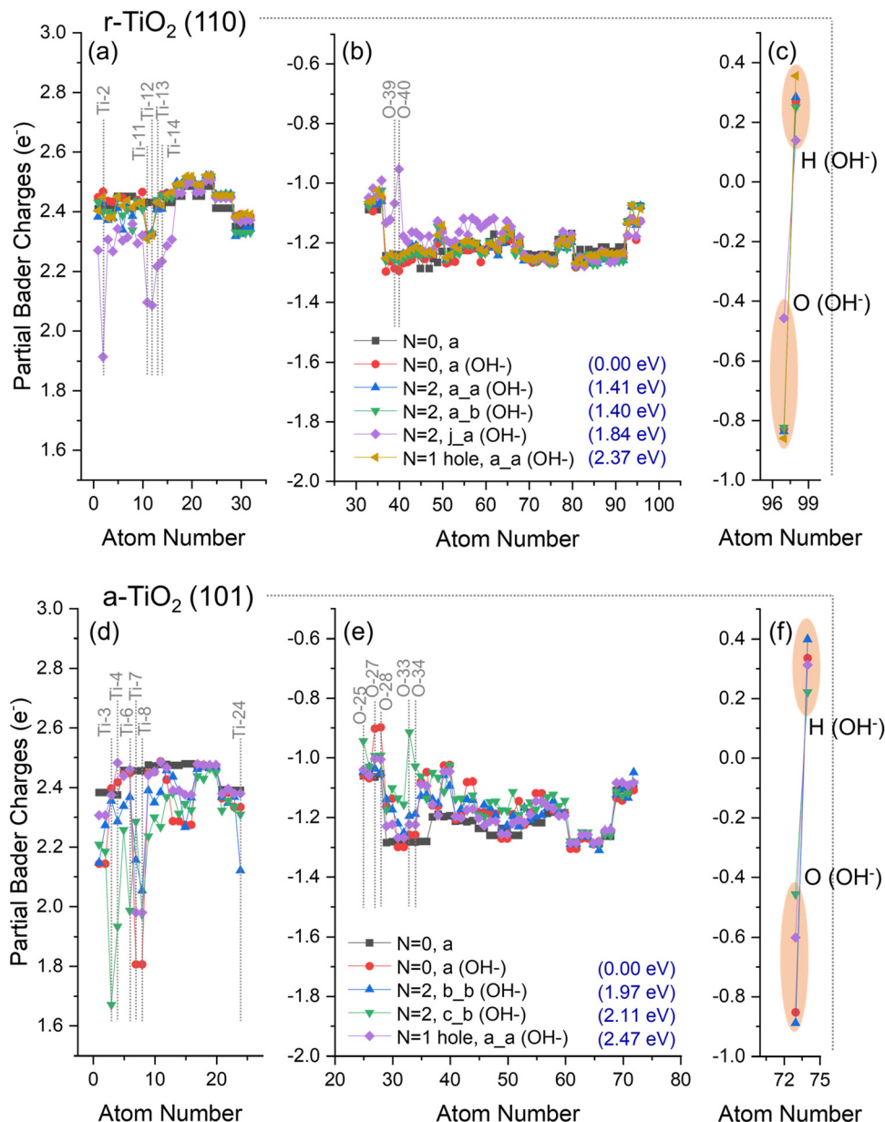
Fig. 6 Partial Bader charges over (a–c) \text{OH}^-/r\text{-TiO}_2 (110) and (d–f) \text{OH}^-/a\text{-TiO}_2 (101) surfaces when considering the ground state ( N = 0 , a; and N = 0 , a ( \text{OH}^- )) of the electronic structure, as well as triplet state ( N = 2 b_b ( \text{OH}^- ) and N = 2 c_b ( \text{OH}^- )) and hole-containing electronic structure ( N = 1 hole, a, ( \text{OH}^- )). Charges of respective clean surfaces are given for comparison. Charges over Ti ions (a and d), O ions (b and e), and adsorbate (c–f) are individually presented. The relative energy ( E_{\text{rel}} ) of each structure is given in parentheses. Atom numbers refer to labels defined in the methodology section.
