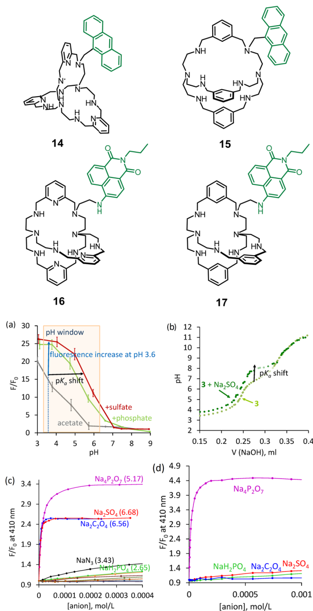
containing azacryptands to detect \text{TcO}_4^- in an acidic aqueous solution. In this work, the heavy-atom containing anion quenches the fluorescence of azacryptands due to the selective encapsulation. 39
