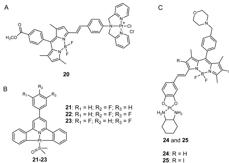
Fig. 5 Lysosome targeted platinum anticancer complexes. The chemical structures of (A) Pt-BDPA ( 20 ); (B) \text{C}^{\wedge}\text{N}^{\wedge}\text{C} ligand-cyclometalated Pt(II) complexes ( 21–23 ); (C) mono-styryl BODIPY-Pt(II) complexes ( 24 and 25 ).
