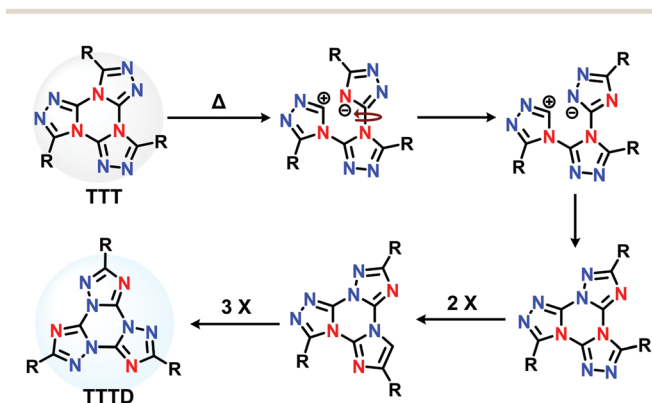
Scheme 1 The isomerization of TTT to TTTD. 35
