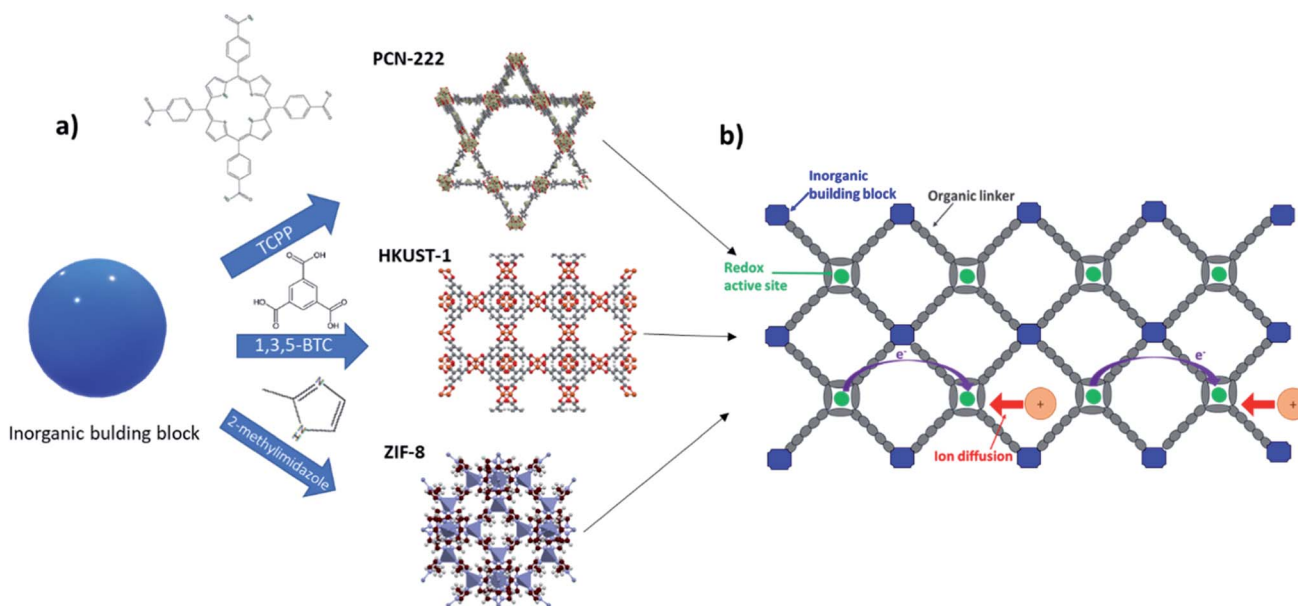
Fig. 2 (a) Diagram showing different MOF families depending on the nature of the linker. MOF structures adapted from ref. 31–33. (b) Scheme of the redox hopping mechanism through the internal MOF structure.
