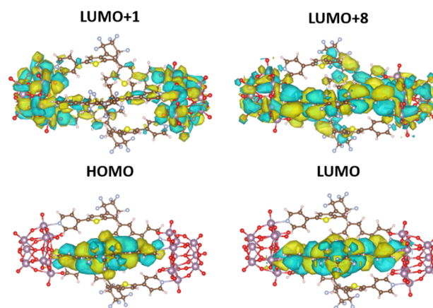
Fig. 7 CAMB3LYP/def2-SVPD 41 orbitals (plotted with standard settings in VESTA) for the most relevant excitations in (\mathbf{1}(\mathbf{O}_A)_2(\text{C})_1) as listed in (Table S6†).
