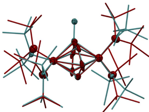
Fig. 5 Overlay of the crystal structures of 5-Li (maroon) and 6-K (teal). Displacement ellipsoids are drawn at the 50% probability level. Hydrogen atoms, NTMS_2 disorder, and counteractions were removed for clarity.
