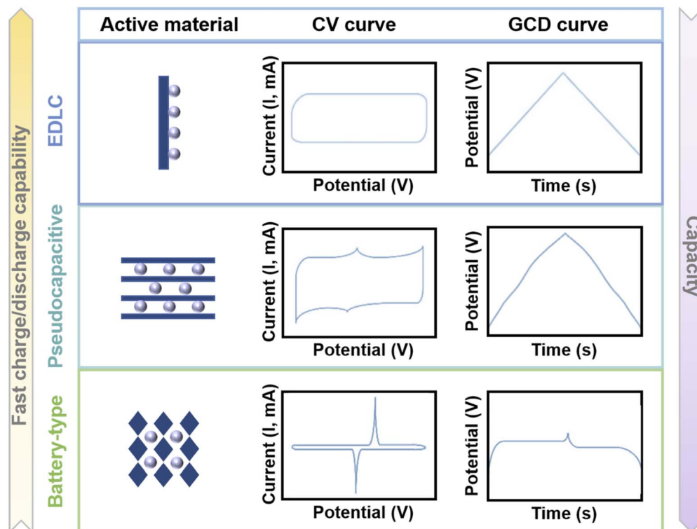
Fig. 2 Illustration of the mechanisms, CV curves and GCD curves of EDLC materials, pseudocapacitive materials, and battery-type materials.
