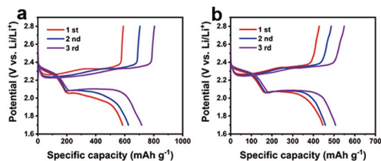
Fig. 5 Galvanostatic charge/discharge curves at 0.1 C rate of (a) CoF 2 -LiF and (b) CoF 2 .
