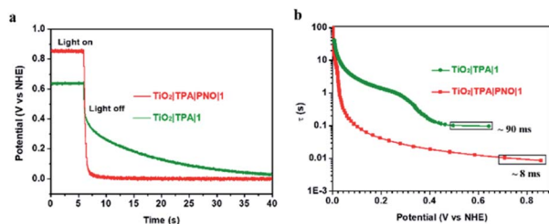
Fig. 9 (a) Open-circuit voltage decays for the electrodes \text{TiO}_2\text{-[TPA|PNO|1]} (red) and \text{TiO}_2\text{-[TPA|1]} electrodes (green). (b) Electron lifetime derived from eqn (7) plotted as a function of V_{\text{oc}} at the transient when illumination ( >400\text{ nm} , 100\text{ mW cm}^{-2} ) was removed. The results were obtained in 0.1\text{ M} phosphate buffer at \text{pH } 7 .
