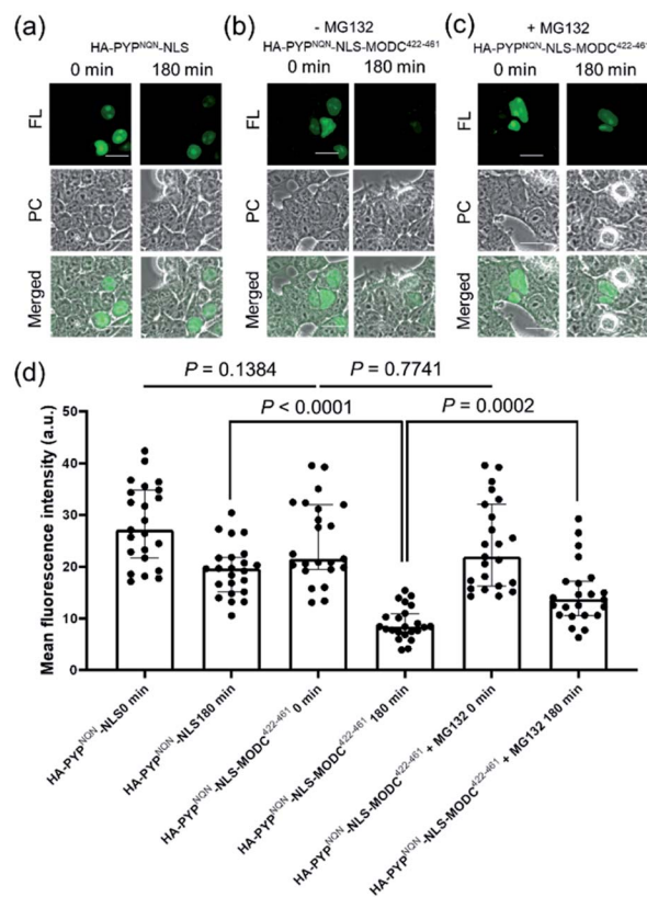
Fig. 8 Use of Ac 2 F 5 -DNB2 (1.0 μM) for the live cell imaging (excitation at 473 nm) of PYP-tagged proteins. (a) Fluorescence images of cells expressing HA-PYP NQN -NLS at 0 and 180 min. (b) Fluorescence images of cells expressing HA-PYP NQN -NLS-MODC 422-461 at 0 and 180 min. (c) Fluorescence images of cells expressing HA-PYP NQN -NLS-MODC 422-461 at 0 and 180 min in presence of 10 μM MG132. Scale bar = 20 μm. PC = Phase Contrast. FL = Fluorescence. (d) Statistical analyses of fluorescence intensities of images of cell nuclei with medians ± interquartile range ( N = 23 cells for each group). Two-tailed unpaired Student's t -test used to show that differences between mean fluorescence intensities for Ac 2 F 5 -DNB2 from the different groups were statistically significant. Data of three independent experiments.
