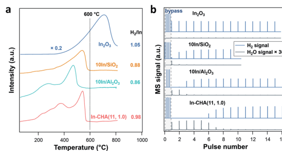
Fig. 2 (a) \text{H}_2 -TPR profiles and (b) results of \text{H}_2 pulse experiments on In-based catalyst at 600 \text{ }^\circ\text{C} .
