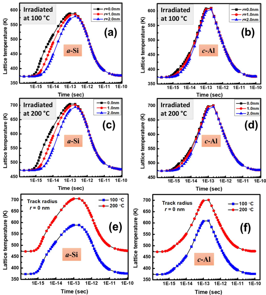
Fig. 9 Thermal spike calculation for the estimation of lattice temperature in (a) a -Si and (b) c -Al due to 100 MeV Ni ion irradiation and for the track radii r = 0, 1, 2 nm when samples irradiated at 100 °C. Lattice temperature in (c) a -Si and (d) c -Al due to 100 MeV Ni ion irradiation and for the track radii r = 0, 1, 2 nm when samples irradiated at 200 °C. (e) Lattice temperature of a -Si at 100 °C and 200 °C. (f) Lattice temperature of c -Al at 100 °C and 200 °C. [Reproduced/adapted from Maity et al. , 157 RSC Adv. , 2020, 10, 4414, with permission from The Royal Society of Chemistry.]
